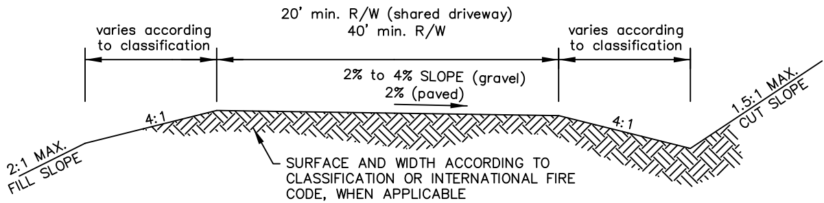
6 A1 PRIVATE ROAD WITH PUBLIC ACCESS
