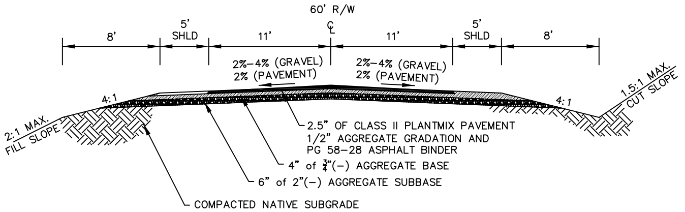
4 A1 RURAL MINOR ACCESS (min. 60' R/W)
