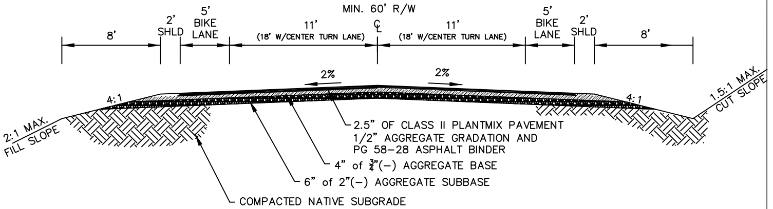
5 A1 RURAL MAJOR ACCESS (min. 60' R/W)
